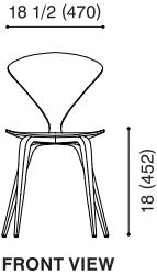
FRONT VIEW
